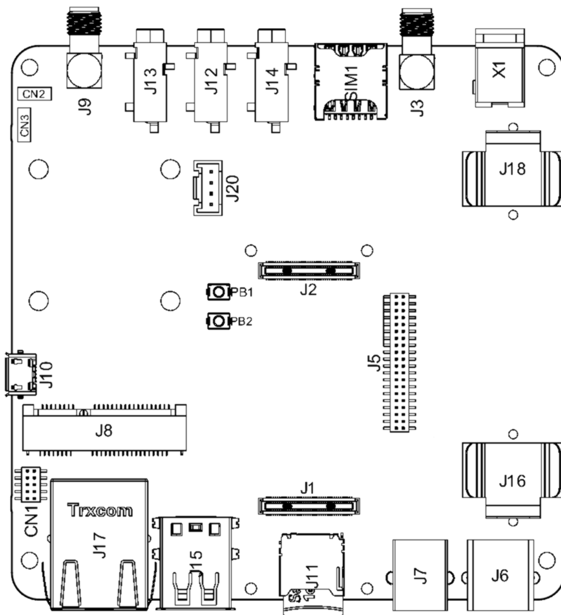
Connectors outline
